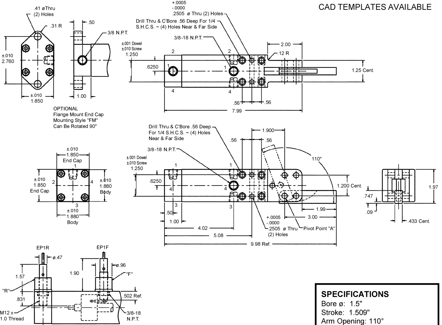
Dimensions For Optional Electrical Proximity Switches
