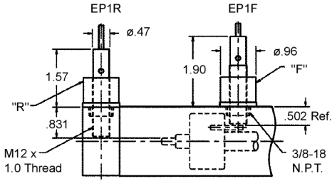
Dimensions For Optional Electrical Proximity Switches
