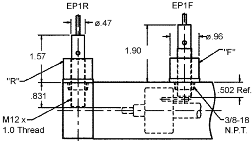
Dimensions For Optional Electrical Proximity Switches
