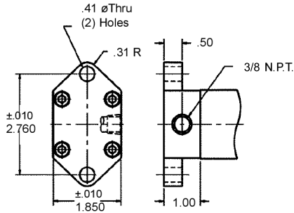
OPTIONAL Flange Mount End Cap Mounting Style "FM" Can Be Rotated 90°
